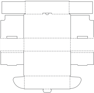
Fefco Code: 0471
